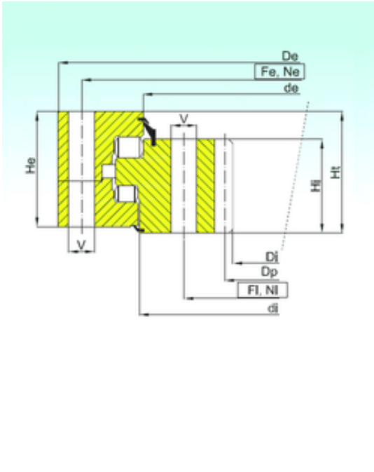
ZR3.25.2000.400-1SPPN Bearing 2D drawings and 3D CAD models
