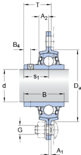
PFT 1.1/2 TR Bearing 2D drawings and 3D CAD models
